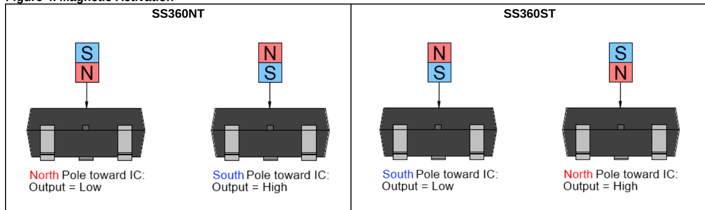
Figure 4. Magnetic Activation
